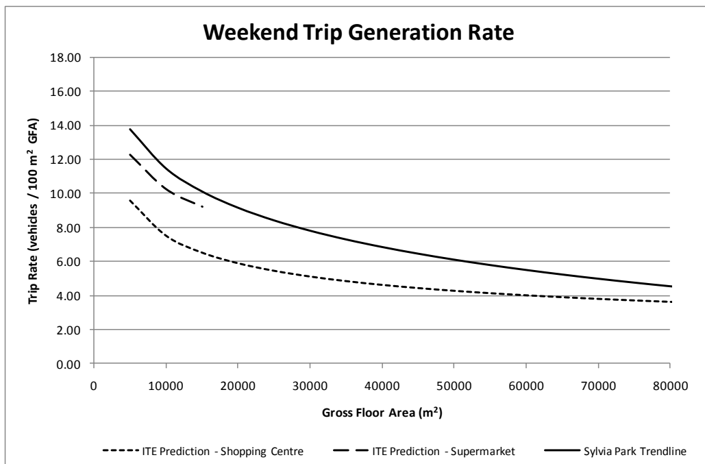
Figure 6: ITE Comparison - Weekend Vehicle Trip Generation Rate
